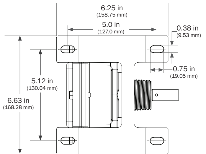
Bottom (base)
