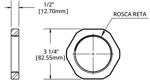
Contraporca LN-51-xx*
