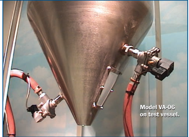
Model VA-06 (with solenoid valve, mounting coupling and lock nut)
